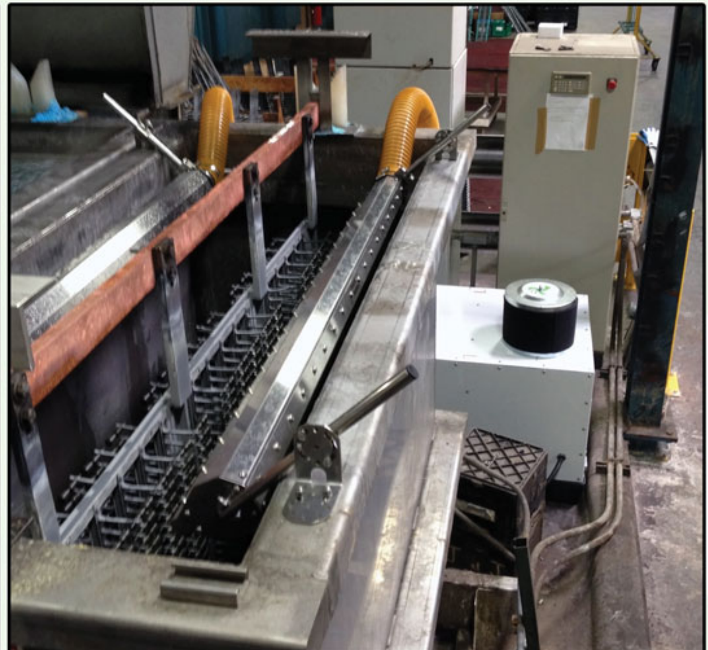
Horizontal “T” Enclosure next to anodizing line
